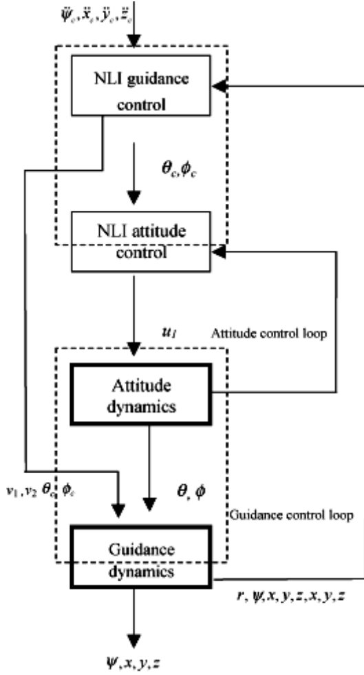
Fig. 2 Proposed control structure
