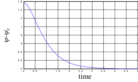
Fig. 4 Heading response during hover
