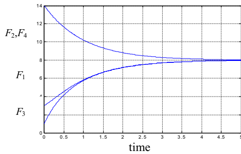
Fig. 7 Rotorcraft trajectory tracking inputs
