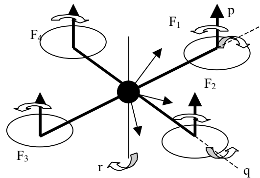
Fig. 1 Four rotor aircraft
