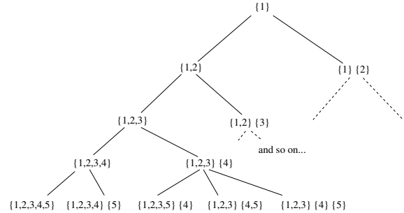
Fig. 2. Searching the partitions of a set of 5 elements
