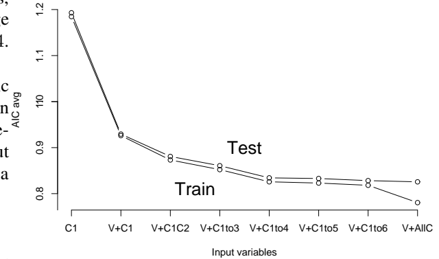
Fig. 3. Values of the AIC_{avg} criterion for the different sets of input variables
