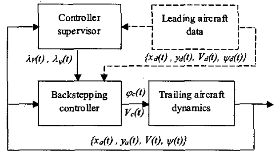
Figure 3. Supervised Controller
