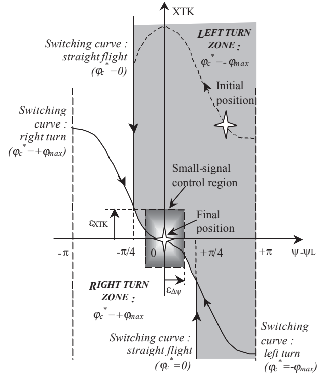
Figure 5 Modified 'cross track' suboptimal control law
