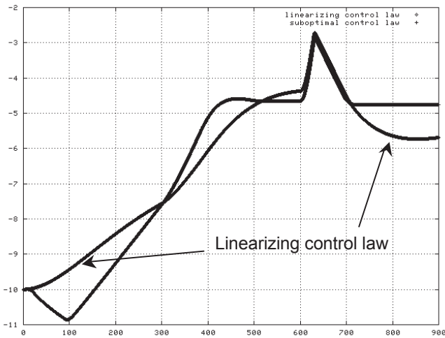
Figure 9 'Along track' distance (TK, in NM) between the leading and the trailing aircraft as a function of time (in sec)
