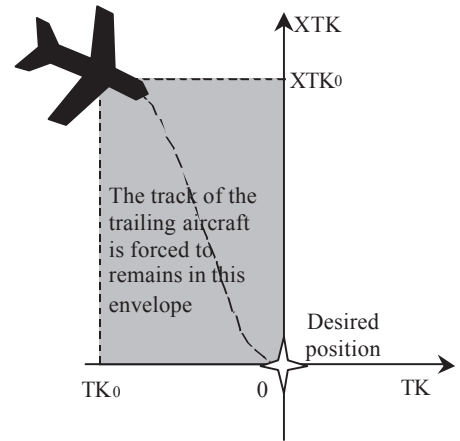
Figure 3 Track envelope of the trailing aircraft
