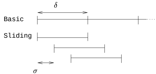
Figure 4: Sliding windows
