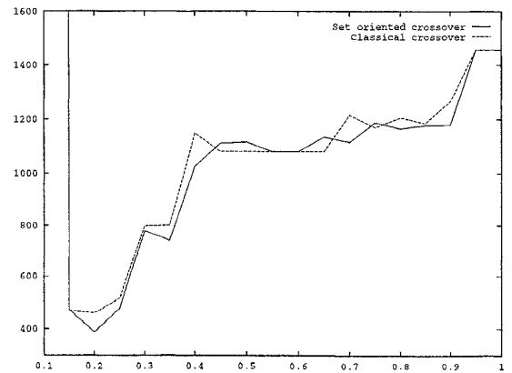
Fig. 2. Influence of \rho on the quality of the solution
