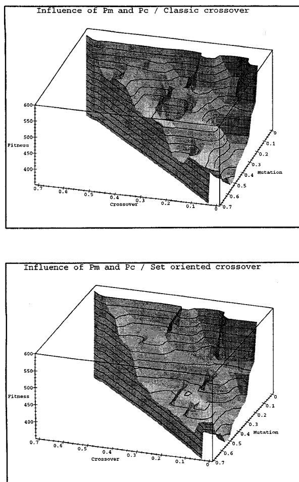
Fig. 3. Influence of crossover and mutation probabilities
