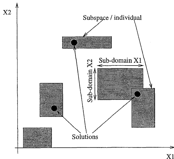
Fig. 1. A two-dimensional search space. The grey rectangles (sub-domains) are the individuals of the GA. Solutions are searched inside these sub-domains by the CSP.
