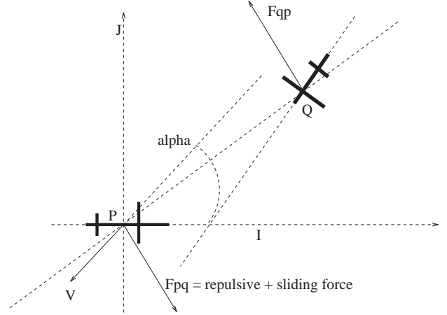
Figure 7: Model for ACAS III logic
