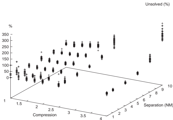
Figure 37: Percentage of remaining conflicts
