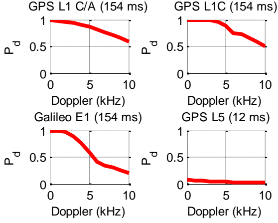
Figure 11: Probability of detection for weak signal and a non-coherent integration on the maximum allowed signal length
