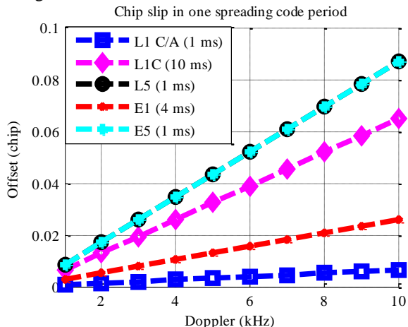
Figure 5: Chip offset in one spreading code period
