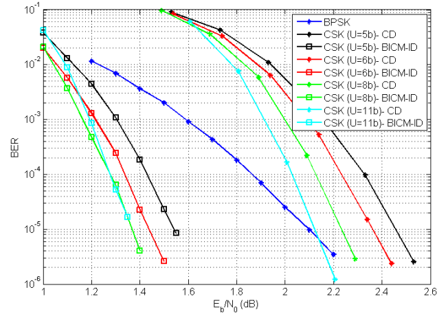
Figure 8: BER vs E_b/N_0 for a reference BPSK signal and for a CSK signal using Classical Decoding method (CD) and Bit-Interleaved Coded Modulation - Iterative Decoding (BICM-IT) with mapping A.
