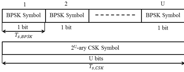
Figure 6: CSK symbol with respect to a BPSK symbol when keeping the coded bit data rate
