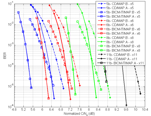
Figure 13: BER vs normalized C/N_0 for CSK signals with increased bit rate with respect to a BPSK signal. CSK signal use Classical Decoding method (CD) and Bit-Interleaved Coded Modulation - Iterative Decoding (BICM-IT) with mapping A and mapping B. All the CSK configurations are defined ( U, N=1 ).
