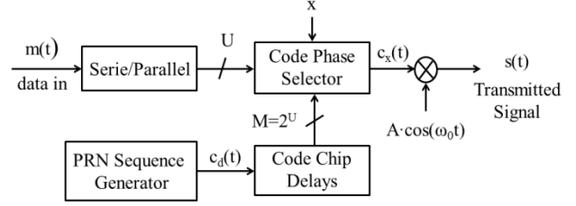
Figure 2: CSK modulator block
