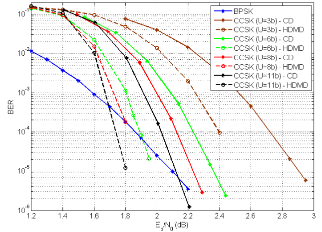
Figure 7: BER vs E_b/N_0 for a reference BPSK signal and for a CSK signal using Classical Decoding method (CD) and Horizontal Dimension Multistage Decoding (HDMD) with mapping A.
