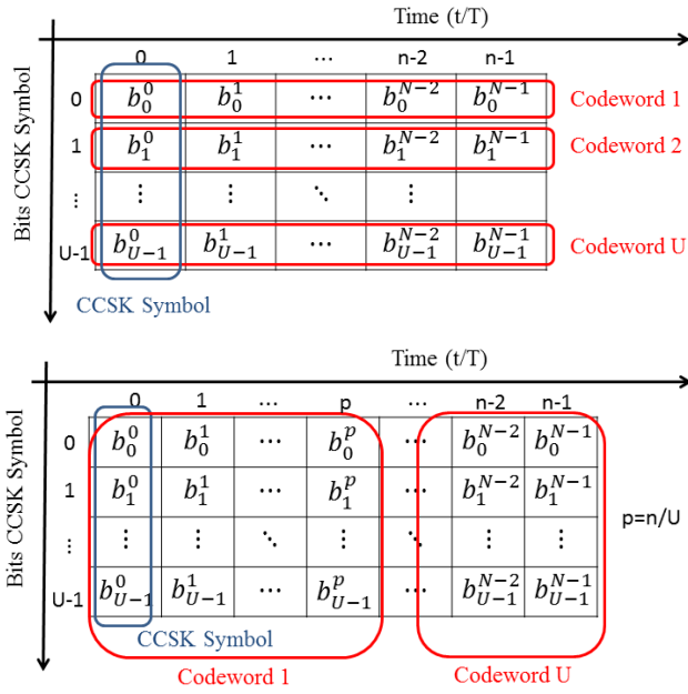
Figure 4: Codeword source mapping A (above) and codeword source mapping B (below) of a CSK modulation
