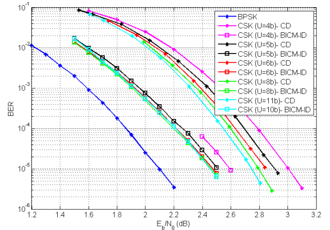
Figure 9: BER vs E_b/N_0 for a reference BPSK signal and for a CSK signal using Classical Decoding method (CD) and Bit-Interleaved Coded Modulation - Iterative Decoding (BICM-IT) with mapping B.
