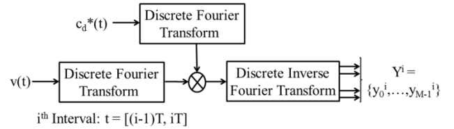
Figure 3: CSK FFT-base demodulator block [12]
