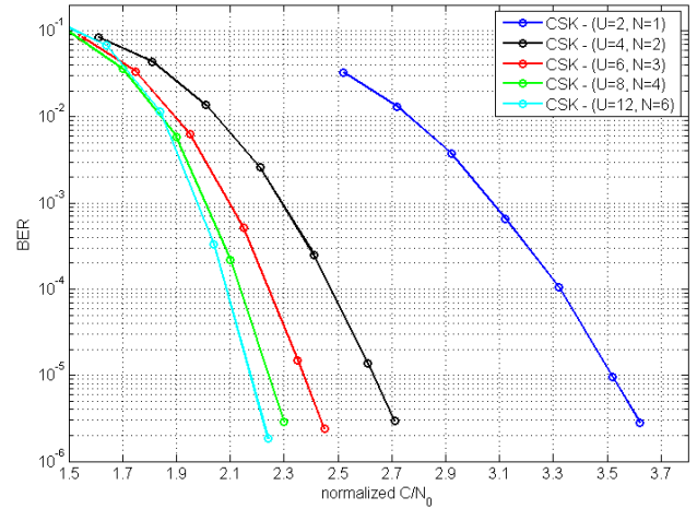
Figure 12: BER vs norm C/N_0 for a different ( U, N ) configuration of a CSK signal using Classical Decoding method (CD) with mapping A when increasing the bit rate by a factor of 2 w/r to a BPSK signal.
