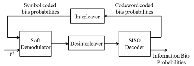
Figure 5: BICM-ID scheme
