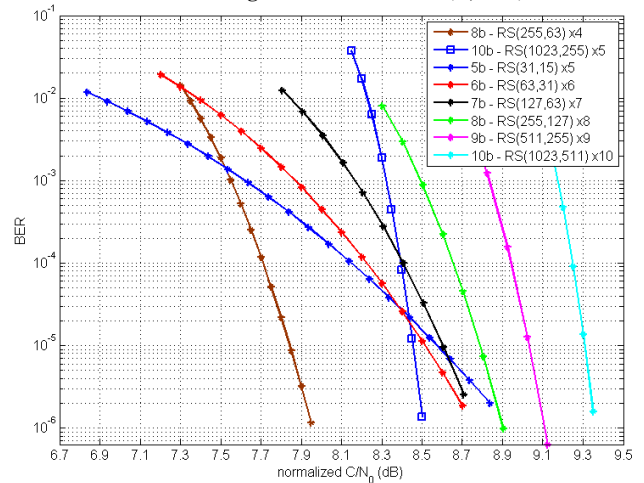
Figure 14: BER vs normalized C/N_0 for CSK signals with increased bit rate with respect to a BPSK signal. CSK signal implement Reed-Solomon (RS) channel codes with code rate equal to 1/2 or 1/4. All the CSK configurations are defined ( U, N=1 ).
