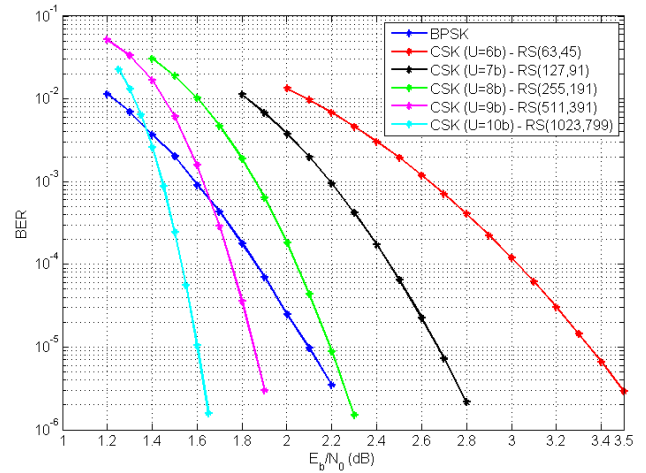
Figure 10: BER vs E_b/N_0 for a reference BPSK signal and for CSK signal with Reed-Solomon channel codes.
