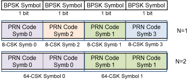
Figure 11: Different possible combinations of CSK symbols producing a bit rate increased by a factor of 3 with respect to the original BPSK signal
