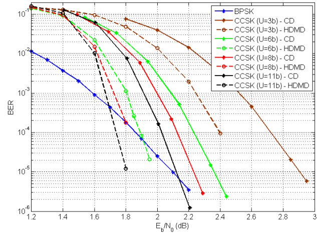
Figure 7: BER vs E_b/N_0 for a reference BPSK signal and for a CSK signal using Classical Decoding method (CD) and Horizontal Dimension Multistage Decoding (HDMD) with mapping A.
