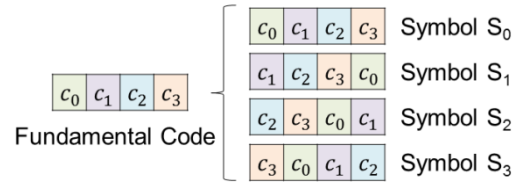
Figure 1: Example of CSK Modulation with M=4 (and U=2 bits)
