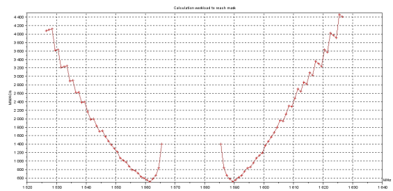
Figure 22. Estimated calculation workload on the E1/L1 band, Separate Sampling
