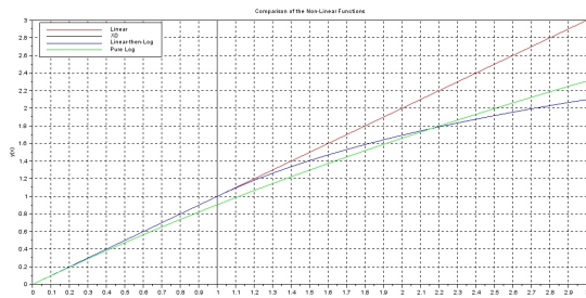
Figure 32. Comparison of the two non-linear functions, close-up
