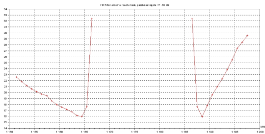
Figure 19. Minimum FIR filter order to reach the required minimum attenuation on the E5a/L5 band, Separate Sampling
