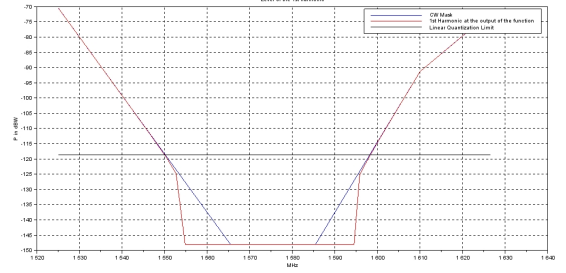
Figure 27. Compression effect of the linear-then-log function on the E1/L1 CW interference mask
