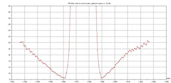
Figure 21. Minimum FIR filter order to reach the required minimum attenuation on the E1/L1 band, Separate Sampling
