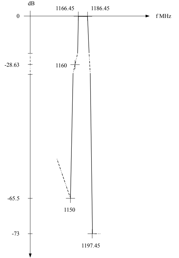
Figure 17. Minimum attenuation to be provided at the output of the ADC in the E5a/L5 band, Separate Sampling
