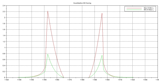
Figure 38. Quantification bit saving offered by the pure log function on the E1/L1 band
