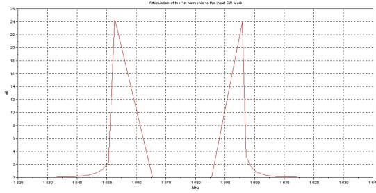
Figure 37. Attenuation provided by the pure log function on the E1/L1 CW interference mask
