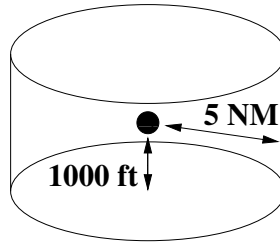
Figure 1 Vertical and horizontal separation: another aircraft cannot be inside the cylinder at the same time.
