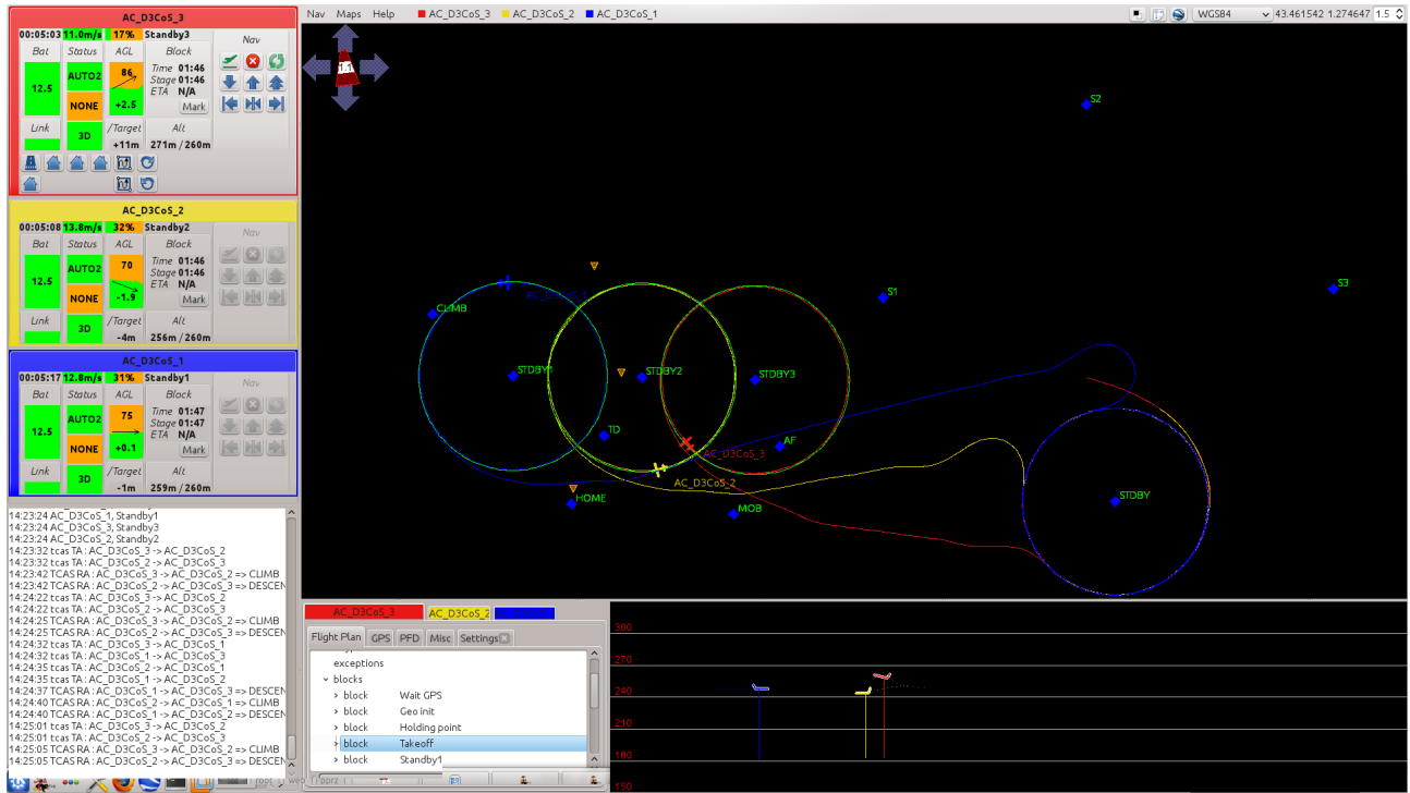
Fig. 5. Planner initialization: 3 aircrafts are circling around their standby points STDBY1, STDBY2, STDBY3 and waiting for the next commands. During flight, Collision avoidance module (using "TCAS") is always triggered each 500 (ms) and the conflict is detected if it happens. In this figure, we can see the conflict between the red and yellow aircraft. As the result, the red aircraft is climbing and the yellow one is descending for avoiding the collision between them. We can see this phase in the altitude interface on the lower side of the figure.
