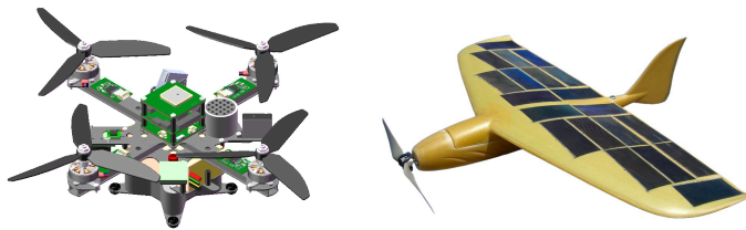
Figure 1. Quadrirotor (Blendeon, 350mm diameter and 300g weight) and aircraft (Solar Storm, 500mm span and 400g weight) min-UAVs from the ENAC (Ecole Nationale de l'Aviation Civile) University
