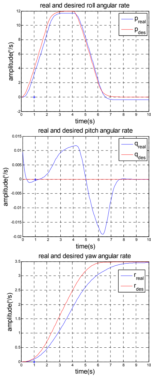
Fig. 12 The real and desired angular rates under hard fault scenario
