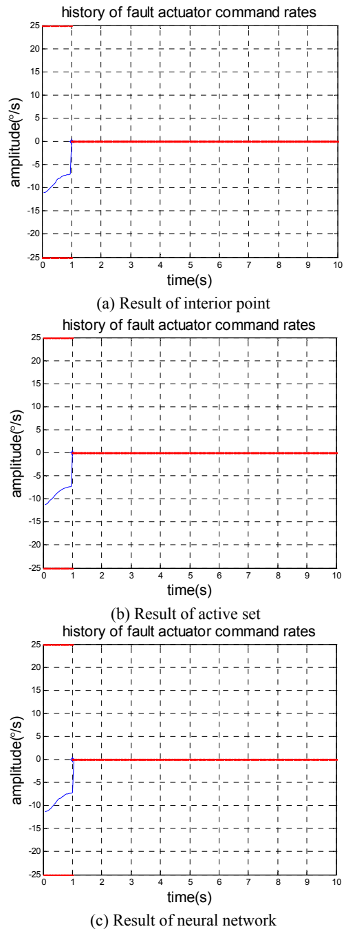
Fig. 13 Command rates for the right outer aileron under hard fault scenario
