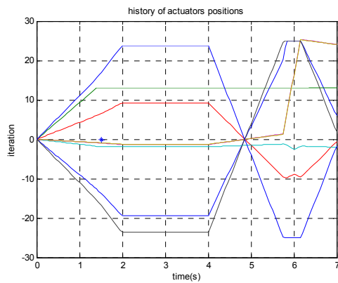
Fig 8. Time evolution of actuators positions under hard fault scenario
