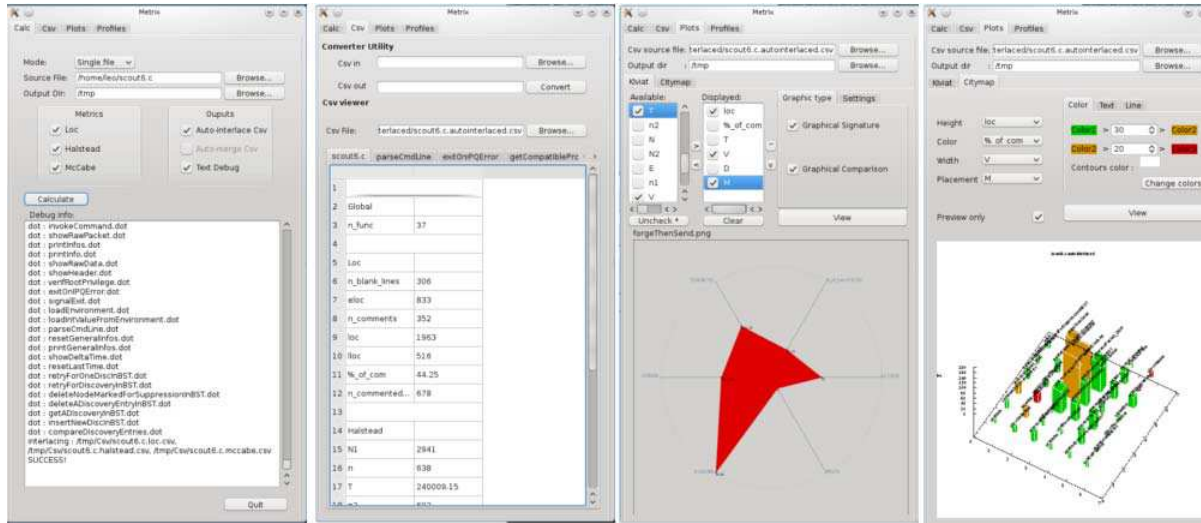
Figure 6. Calc and Csv tabs of the Metrix GUI at left, "Plots" tab of METRIX GUI to represent Kiviati and city maps at right
