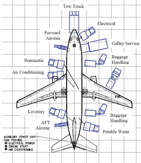
Figure 2: Ground handling arrangement [2] .
