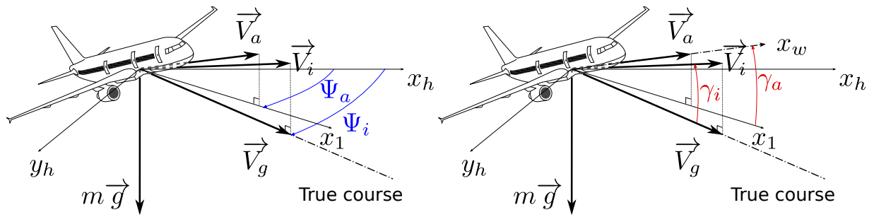
Figure 2: \Psi and \gamma angles (with x_h pointing to the North)
