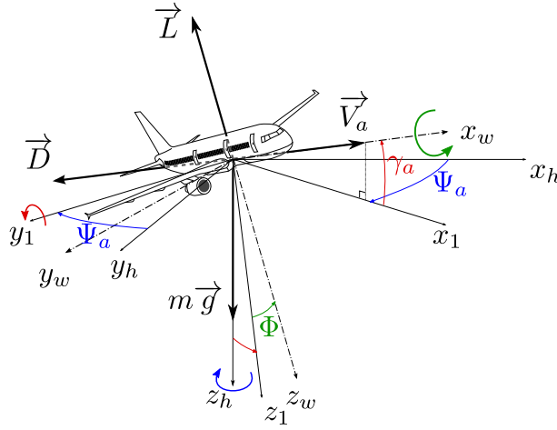
Figure 1: Euler rotations of angles ( \Psi_a, \gamma_a, \Phi ) with counter-clockwise convention, and right-handed coordinate systems.
