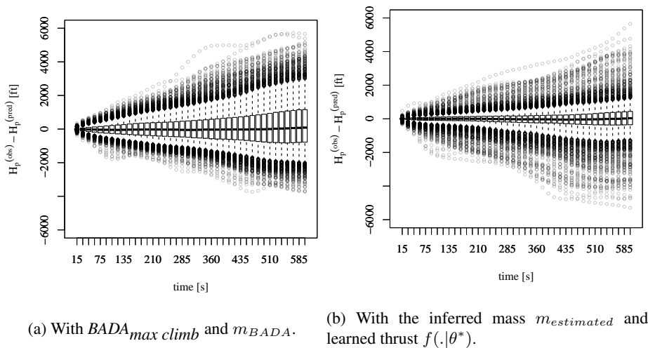
Figure 6: Altitude errors (case study 2) for future times from 15 s to 10 mn.
