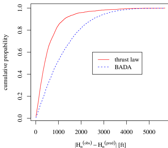
Figure 7: Empirical cumulative distribution of the altitude errors 10 minutes ahead, for the BADA model (blue dotted curve) and our method (red solid curve).
