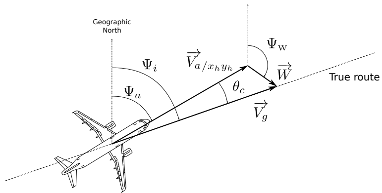
Figure 3: Angles in the local horizontal plane
