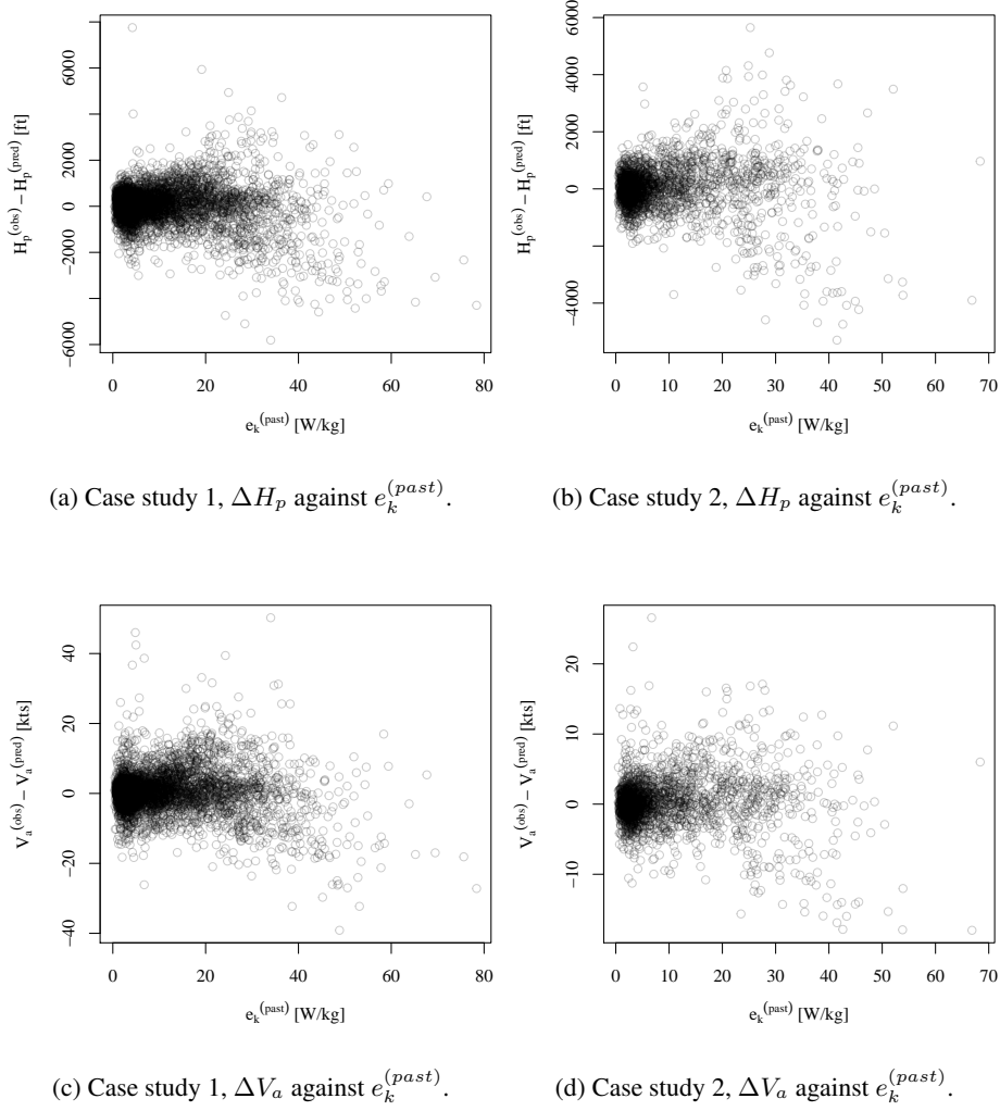
Figure 8: Relationship between e_k^{(past)} and the altitude and velocity errors at the last point of the prediction.
