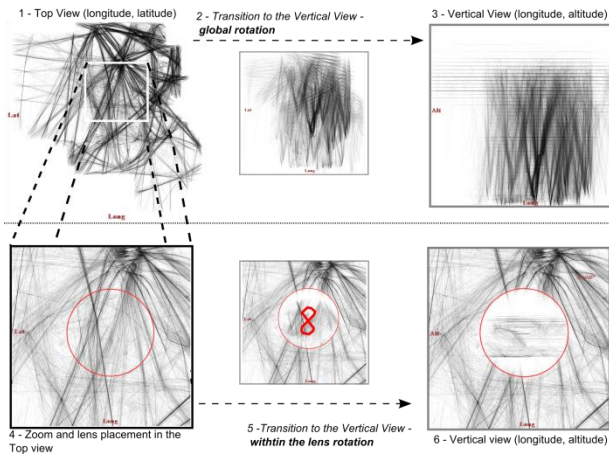
Figure 7: The user switches from a top (1) to a vertical (2,3) view. In the top view, the user selects graphical marks with the lens (4). During the 3D rotation within the lens, the user perceives that the noticeable trajectory depicts an “8” (5).
